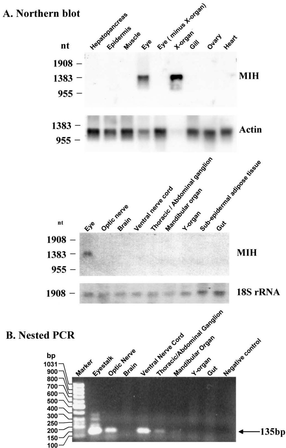
Fig. 4. Tissue distribution of MIH mRNA. (A) Northern blot showing tissue distribution and size of the C. pagurus MIH transcript. Approximately 10 \mu g of total RNA from a variety of C. pagurus tissues and two organ equivalents of X-organ RNA was electrophoresed, blotted onto a nylon membrane, hybridised at 68°C with a ^{32} P-labelled- MIH probe A (nucleotides 220–1314) and washed at 60°C. Blots were re-hybridised under the same conditions using a \beta -actin cDNA probe from crayfish (Kang and Naya, 1993) or a mouse 18S rRNA probe (Chen et al., 1999). (B) Nested PCR analysis of C. pagurus tissues for the presence of MIH transcripts. Two \mu g of total RNA from a variety of tissues was used as template for synthesis of first-strand cDNA. The cDNA was used, in turn, as template for nested PCR using MIH sequence-specific primers to amplify a 135 bp MIH fragment.
