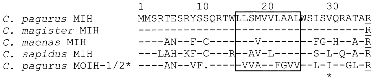
Fig. 2. Comparison of signal peptides of CHH family members. Direct alignment of amino acid sequences of signal peptides from Cancer pagurus MIH, Cancer magister MIH (Umphrey et al., 1998), Carcinus maenas MIH (Klein et al., 1993), Callinectes sapidus MIH (Lee et al., 1995) and C. pagurus MO-IH-1 and -2 (Tang et al., 1999) is given. A gap (dot) has been introduced into C. pagurus MO-IH-1/2 to maximise alignment. The hyphens denote identical amino acids to C. pagurus MIH. The boxed area outlines a core of hydrophobic amino acids common to signal peptides. The asterisk indicates a substitution of I in MO-IH-1 for S in MO-IH-2. The first amino acid of each mature peptide is underlined.
